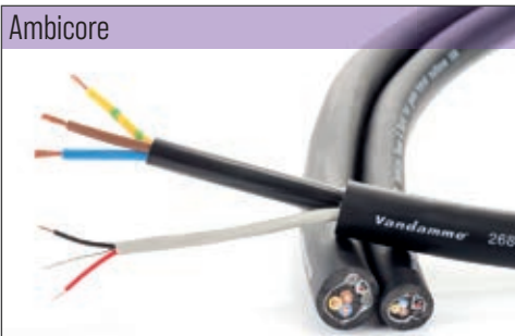
Power & Signal Tour Grade 15A 3 x 1.5mm
